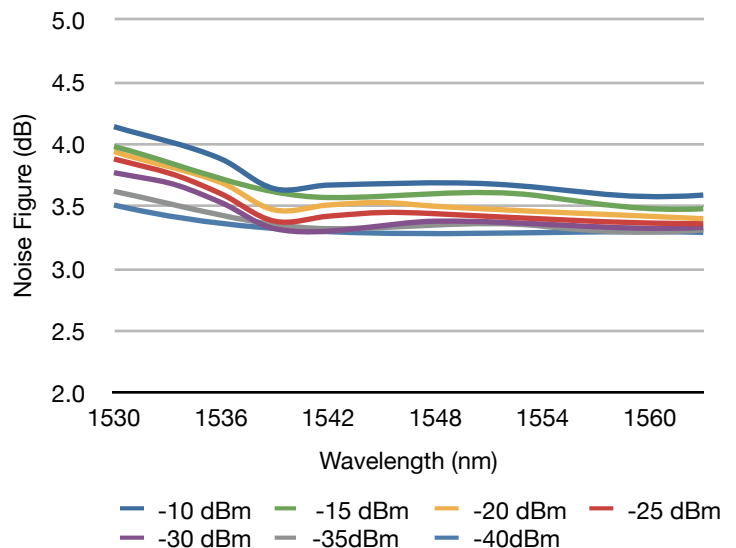
AEDFA-PA-35-B-FA Noise Figure
