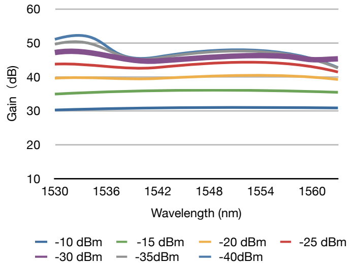
AEDFA-PA-35-B-FA Gain
