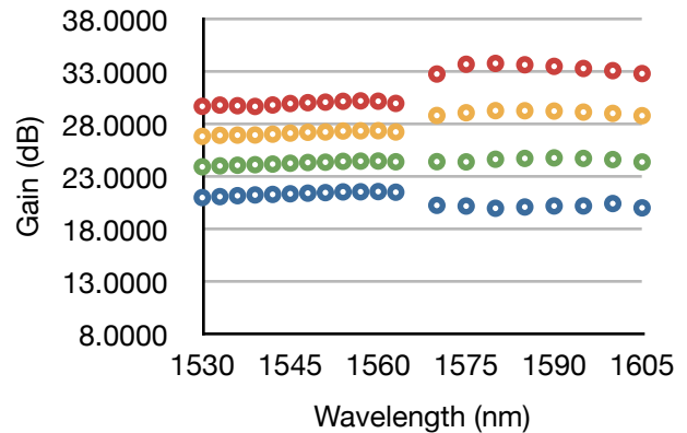
AEDFA-CL-23-B-FA Gain
